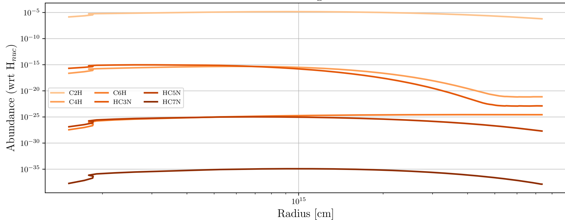
Particle 8286 - Daughter Molecules
