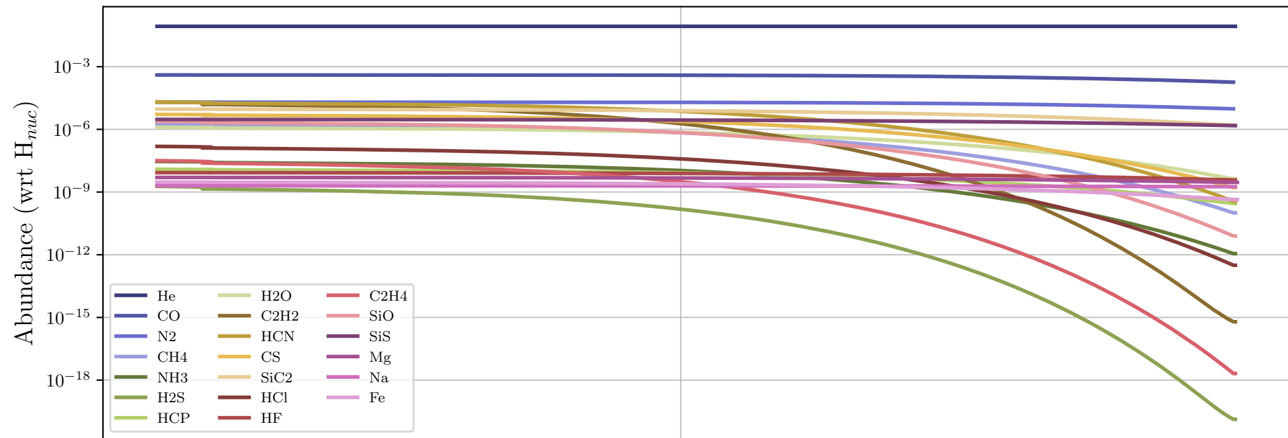
Particle 8286 - Parent Molecules
